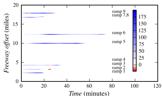
(b) Queue difference profile in units of vehicles.
