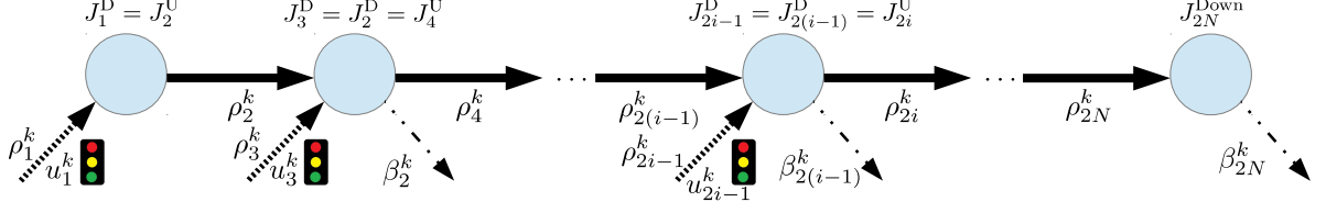
Fig. 5: Freeway network model. For a junction J_{2i-1}^D = J_{2(i-1)}^D = J_{2i}^U at time-step k \in \{0, \dots, T-1\} , the upstream mainline density are represented by \rho_{2(i-1)}^k , the downstream mainline density by \rho_{2i}^k , the on-ramp density by \rho_{2i-1}^k , and the off-ramp split ratio by \beta_{2(i-1)}^k .
